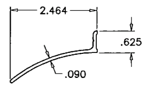
40 DRIP CAP
